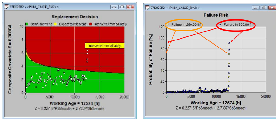
Figure 1: EXAKT Replacement Recommendation Figure 2: EXAKT Probability of Failure
